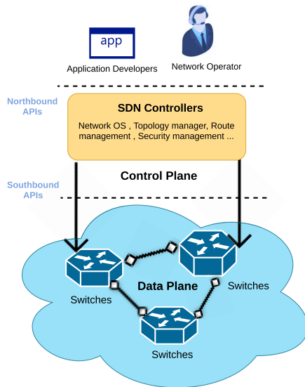
FIGURE 4. SDN-Based network.
