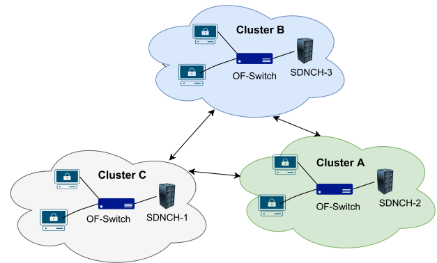
FIGURE 31. SDN-Based Security Framework in Distributed Grid.
