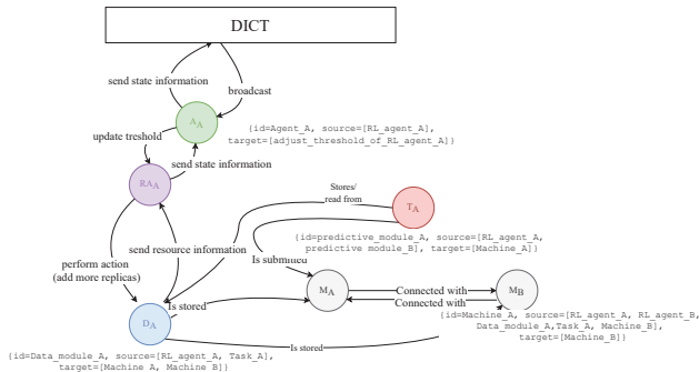
Fig. 3: Illustrative pipeline for the local DICT coordinator and its interaction with the submodules
