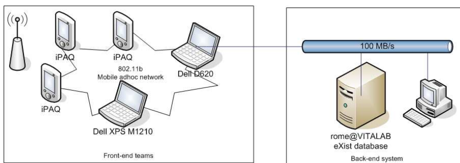
Fig. 5. Testbed deployment
