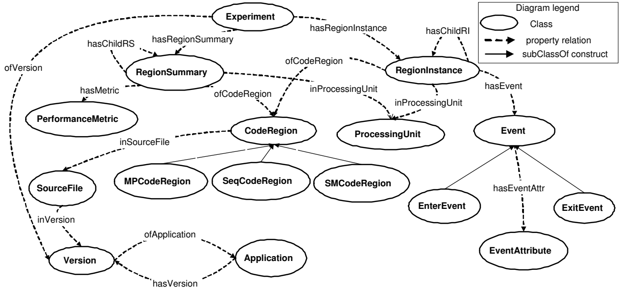
Figure 1: Illustrative classes and properties of experiment-related concepts. subClassOf construct allows to define a class as a subclass of another class. Property relation represents the relation between classes.
