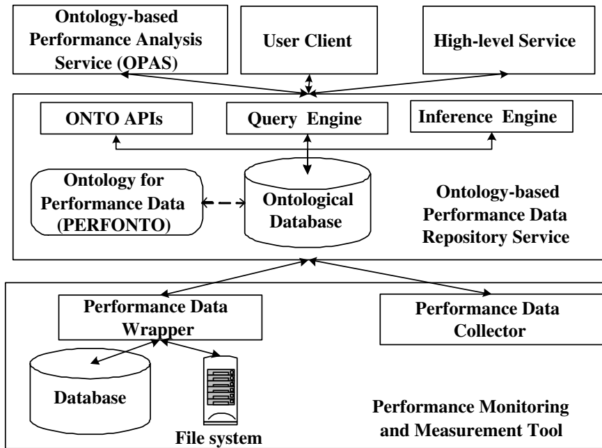
Figure 3: Three layers architecture for an ontology-based model for performance analysis, data sharing and tools integration.
