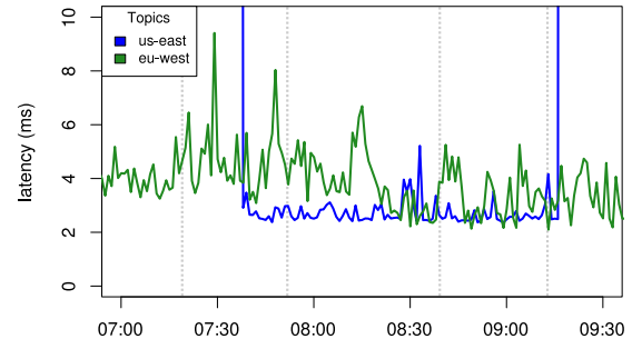
(c) Latencies during intra-region communication
