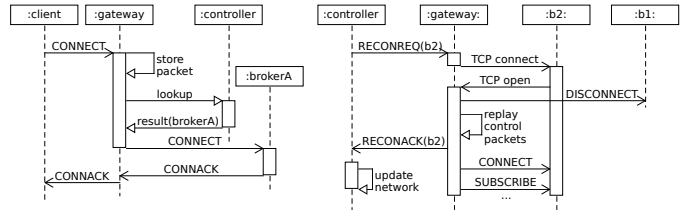
Fig. 2: Connection (left) and reconnection (right) procedures
