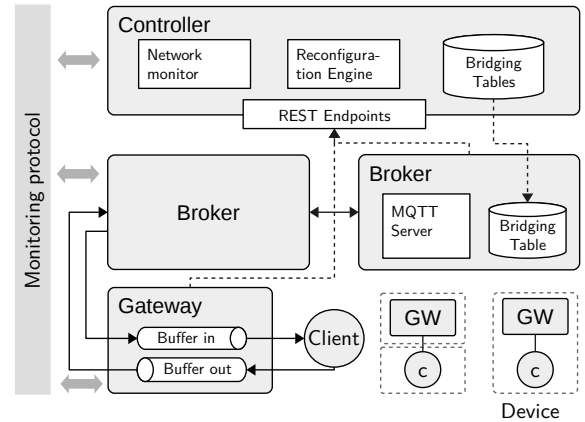
Fig. 1: Overview of the EMMA architecture
