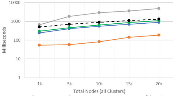
Fig. 5: Mean Scheduling Times (ms) at C_p = 50\% and N_p = 4\% for Total Nodes.
