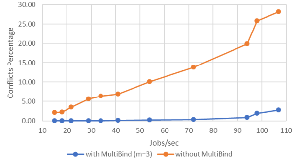
Fig. 9: Scheduling Conflicts with and without MultiBind.
