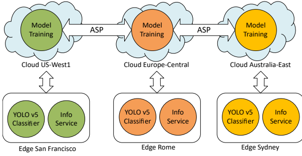
Fig. 1: Globally Distributed Machine Learning.
