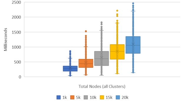
Fig. 8: End-to-End Times (ms), without Sampling Queue, at C_p = 50\% and N_p = 4\% for Total Nodes.
