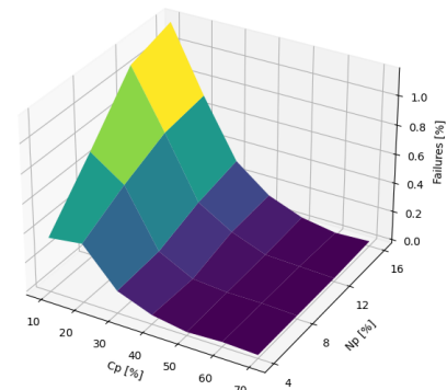
Fig. 4: Scheduling Failure Percentages for Configuration Tuning.
