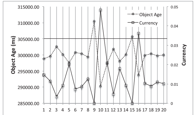
Fig. 5. Feed 3824.2, object currency
