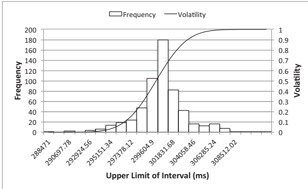
Fig. 3. Feed 3824.2, histogram and volatility
