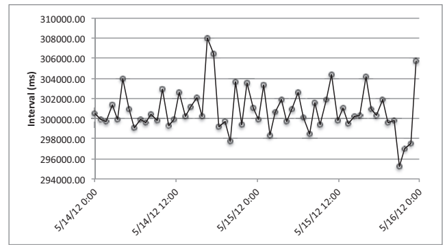
Fig. 2. Feed 3824.2, update interval
