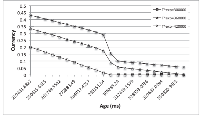
Fig. 4. Feed 3824.2, currency changes with different T^{exp}
