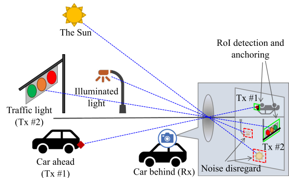
FIGURE 2. RoI detection and anchoring in the next-generation OCC.
