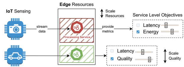
Fig. 1: Processing IoT data at resource-constrained devices; if SLOs are violated, scale either resources or service quality
