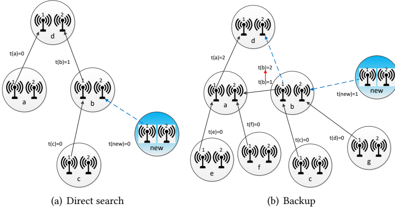
Fig. 7. New nodes joining.
