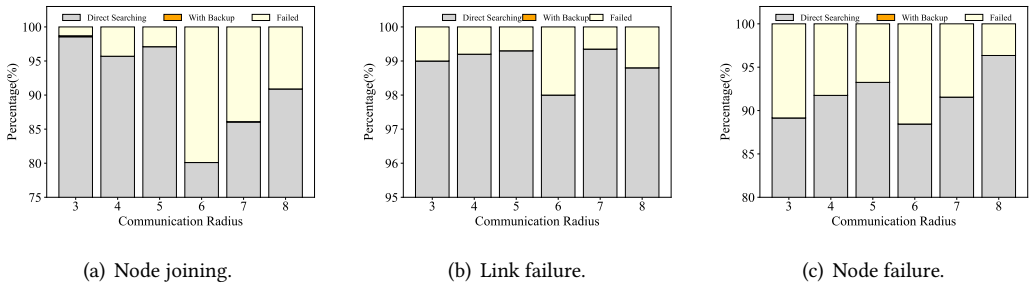
Fig. 11. Result analysis of handling dynamic changes in network topology.
