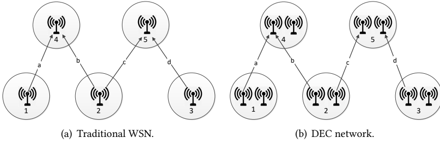
Fig. 1. Interference models of DEC network and the traditional WSN.
