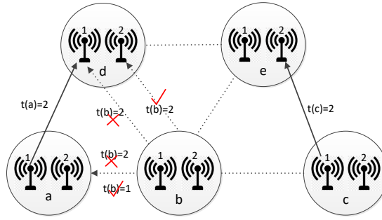
Fig. 3. The example of scheduling.
