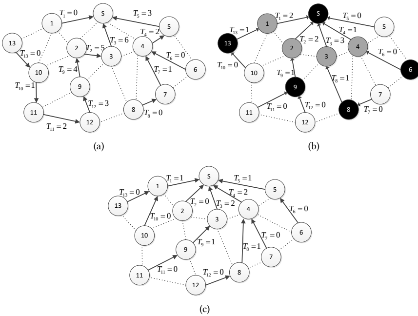
Fig. 2. Data aggregation latency in a DEC network in which each node has two antennas.
