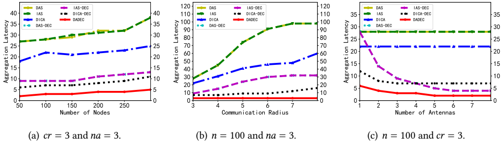
Fig. 8. Aggregation latency in small DEC networks.
