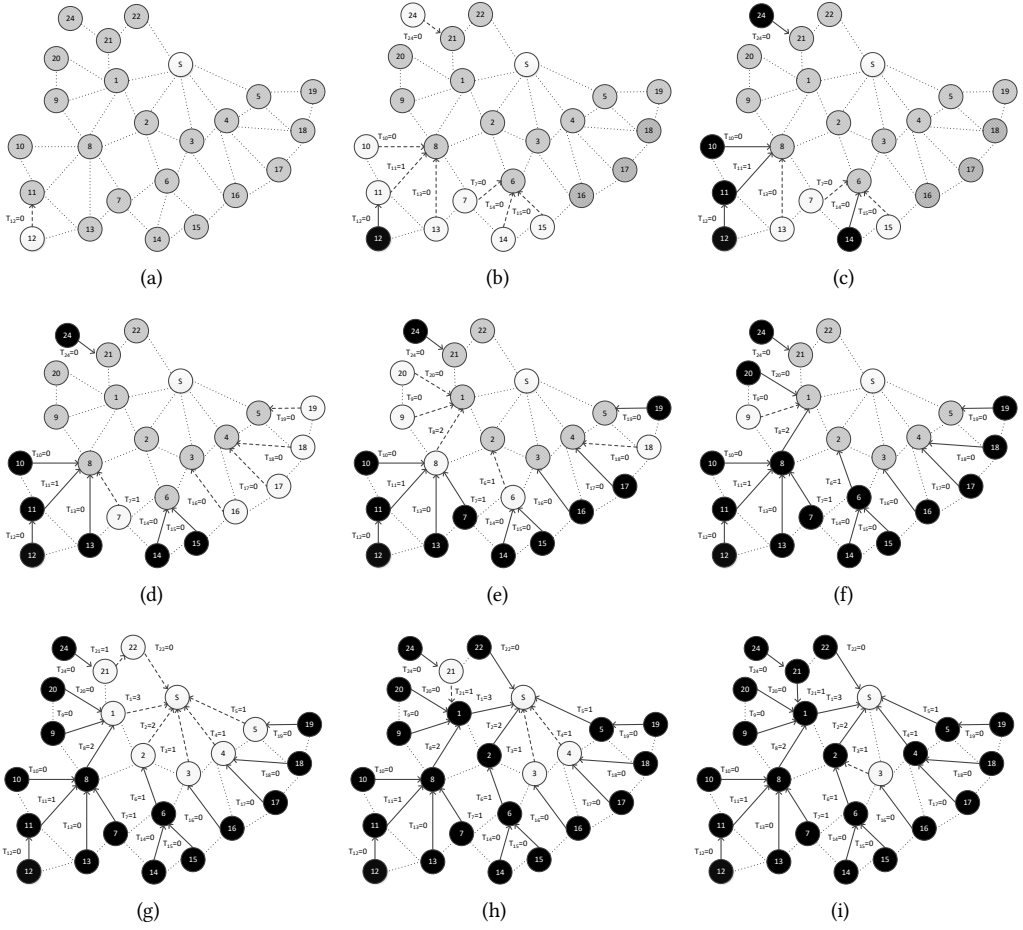
Fig. 5. A representative example of DADEC execution.
