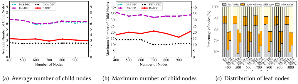
Fig. 10. Node distribution in an aggregation tree.
