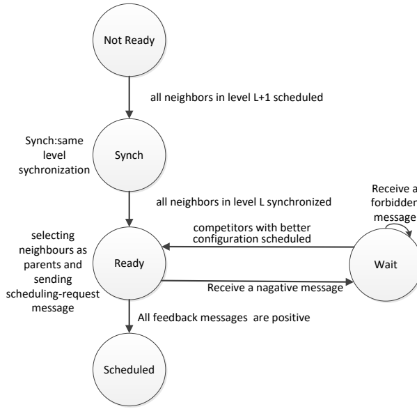
Fig. 4. State transitions of node scheduling.
