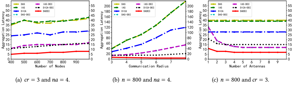
Fig. 9. Aggregation latency in massive DEC networks.
