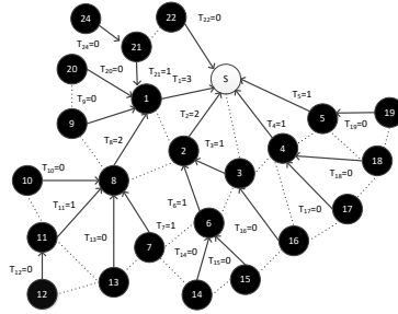
Fig. 6. The execution result of the representative example.
