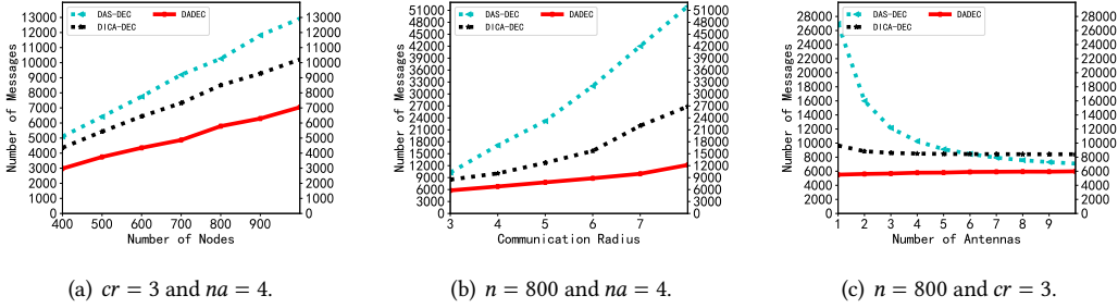
Fig. 12. The number of exchanged messages.
