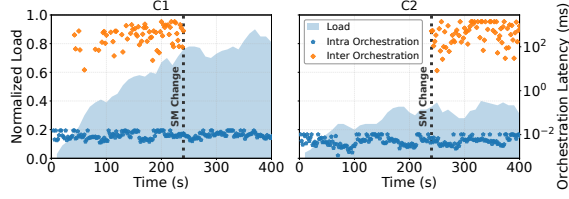
Fig. 4: Super-master behavior under increasing cluster load.
