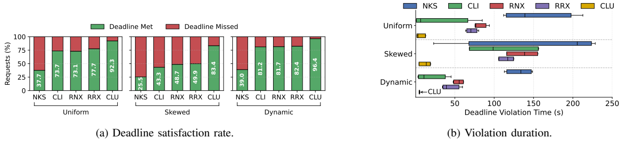
Fig. 7: Deadline violation behavior across strategies and arrival rates.
