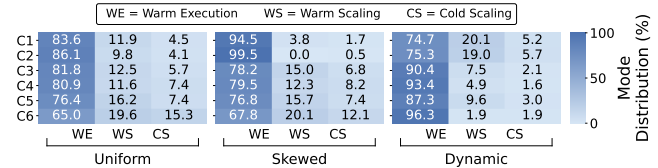
(b) Execution-mode distribution of ClusterLess.
