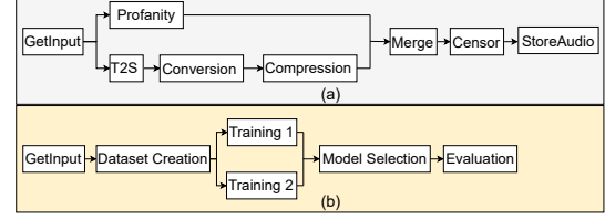
Fig. 2: Case study serverless workflows.
