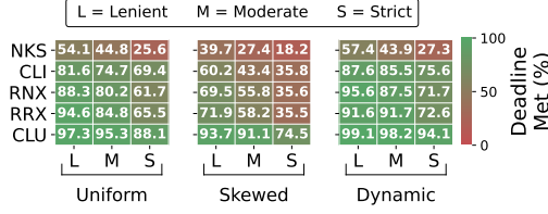
(a) Deadline satisfaction by deadline strictness.
