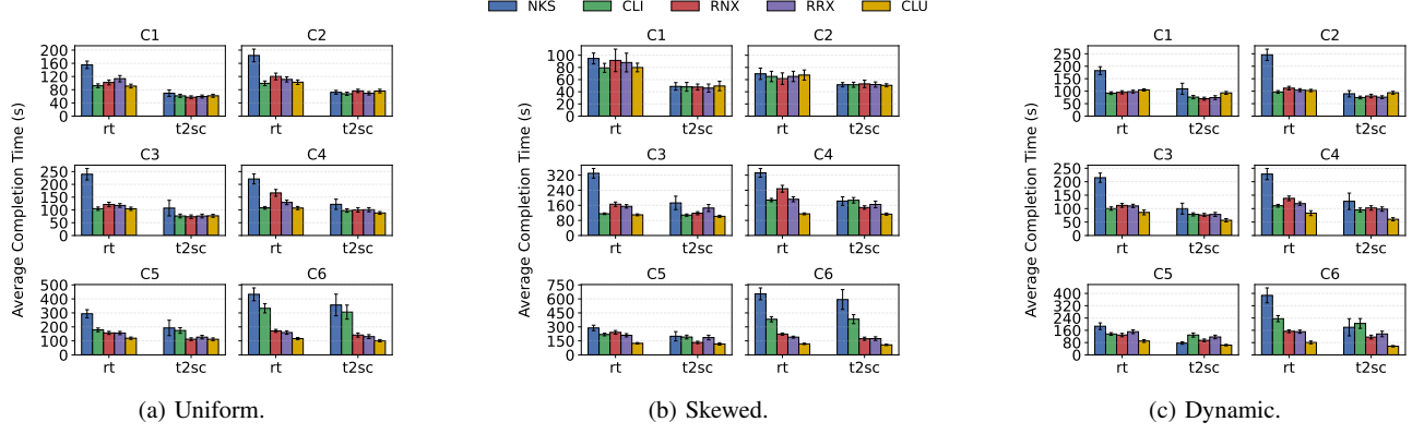
Fig. 6: Average workflow completion time per cluster under different arrival regimes.
