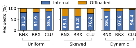
(a) Local vs. offloaded function execution.
