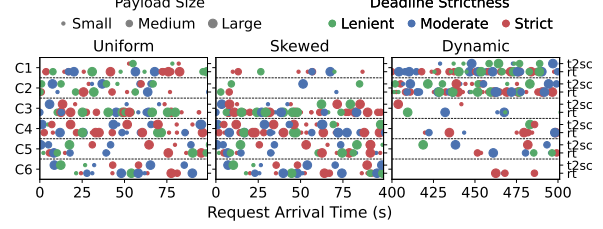
(b) Workflow arrival times per cluster.
