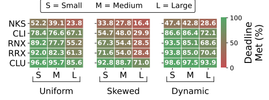
(b) Deadline satisfaction by payload size.
