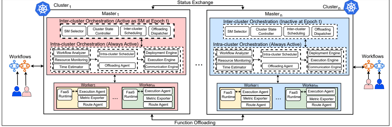
Fig. 1: ClusterLess system architecture.
