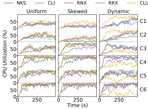
Fig. 10: Per-cluster CPU utilization in different methods.
