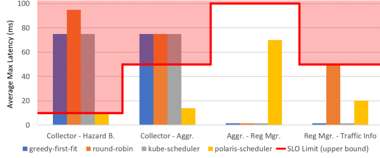
Figure 5.6: Average Max Latencies Achieved by Schedulers and SLO Bounds.
