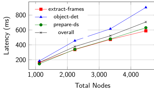
Figure 8.7: HyperDrive Scheduling Latency Across Infrastructure Sizes.
