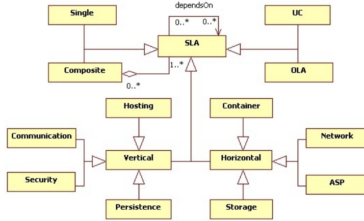
Fig. 7. SLA Categorization.
