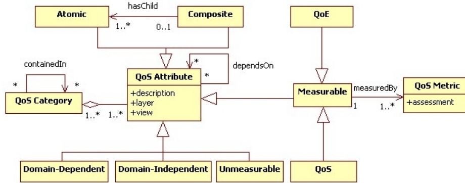
Fig. 4. Ideal meta-model for SQMs.
