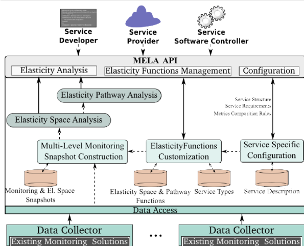
Figure 5 MELA overview (see online version for colours)
