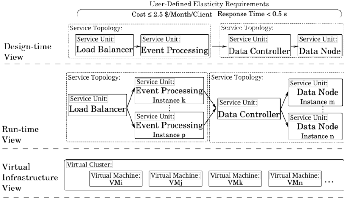
Figure 2 Elastic cloud service views
