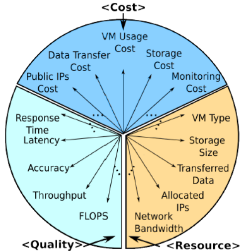
Figure 3 Elasticity dimensions (see online version for colours)
