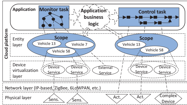
Fig. 1: Example of a cloud-scale IoT application.
