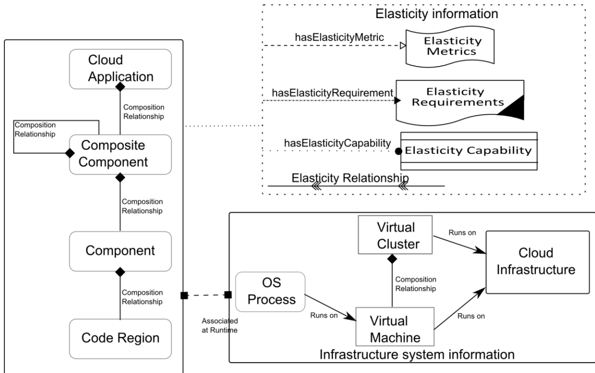
Figure 3: Abstract Composition Model
