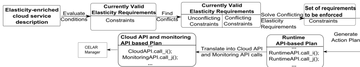
Figure 10: Elasticity Control: from Directives to Action Plans
