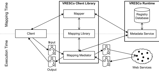
Fig. 7. VMF architecture.
