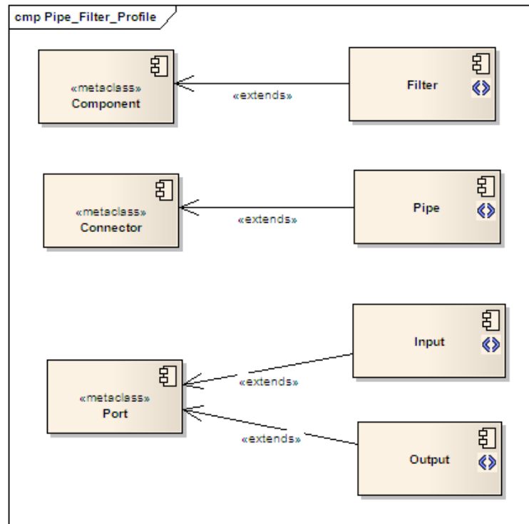
Figure 5. UML stereotypes for expressing Pipes and Filters pattern participants
