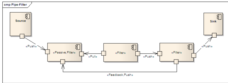
Figure 6. Modeling Pipes and Filters Pattern Variant Using Primitives
