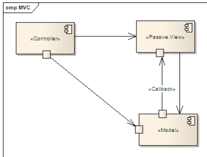
Figure 7. Modeling MVC Pattern Using Primitives
