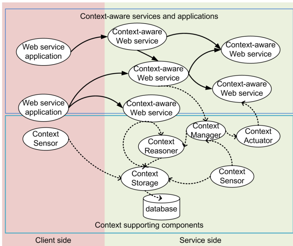
Figure 1: Basic components in a Web service-based context-aware system. Arrowed black lines indicate invocations between applications and Web services. Arrowed dash lines indicate invocations between Web services and supporting components.
