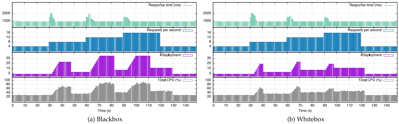
Fig. 4. Evaluation results—IoT application topology optimization (step load pattern).
