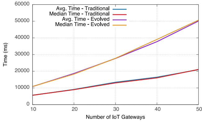
(a) Application Deployment - Deployment Time
