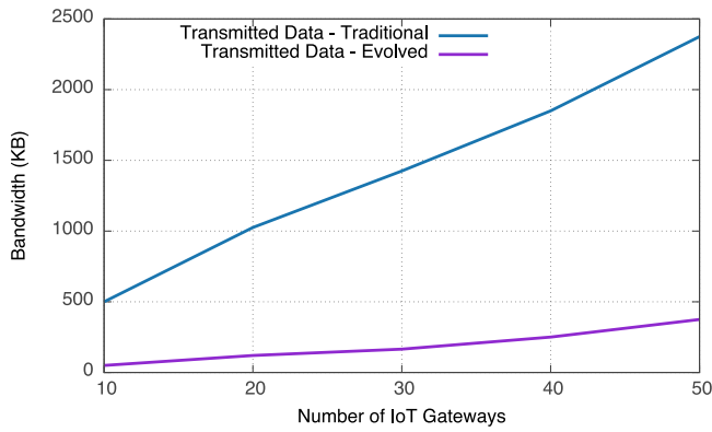
(c) Application Execution - Bandwidth
