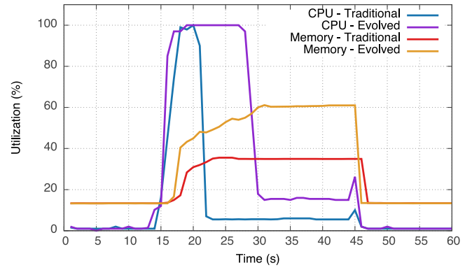
(b) Application Deployment - Device Utilization
