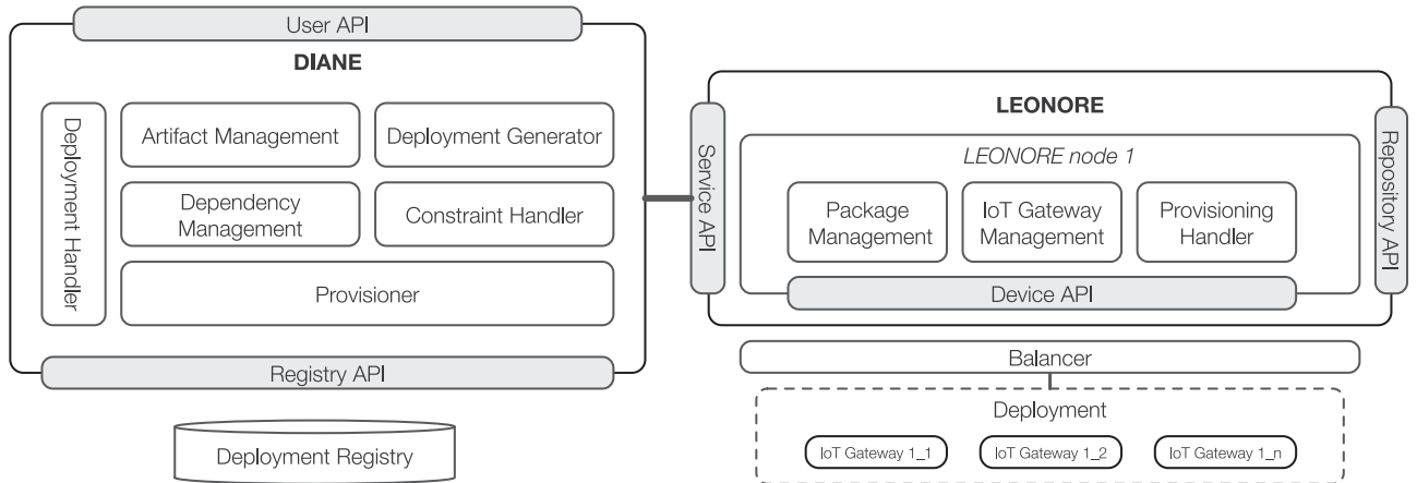
Fig. 1. DIANE and LEONORE—overview.
