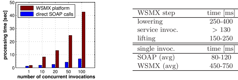
Fig. 9. WSMX performance comparison.
