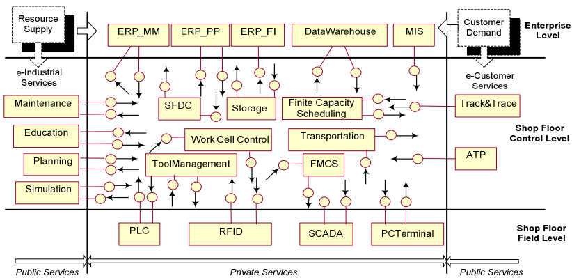
Fig. 1. Internal and external service providers at the shop floor control level
