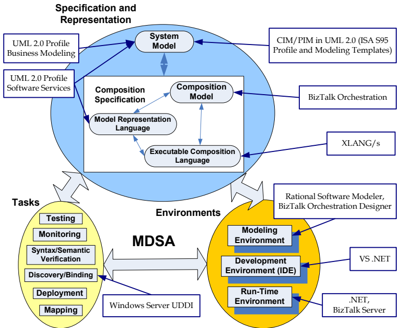
Fig. 3. MDSA implementation
