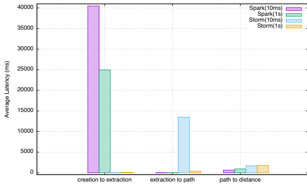
Fig. 6: Latency between processing steps
