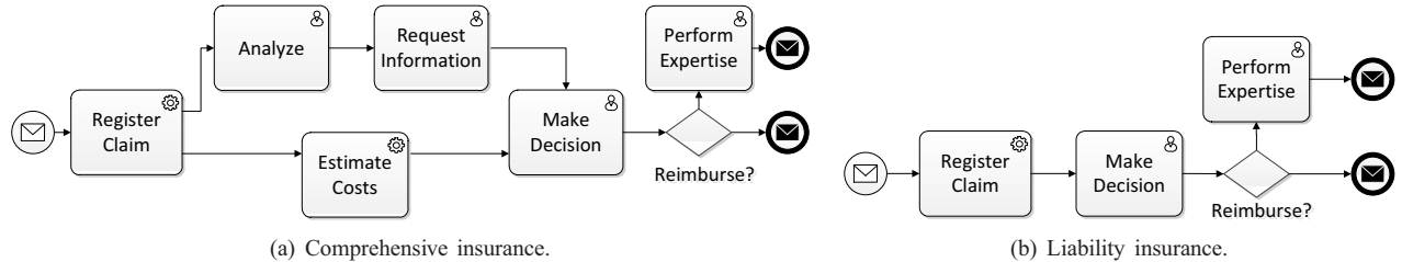
Figure 1. Claim processes for different insurance cases.
