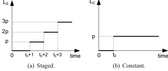
Figure 5. Penalty functions.
