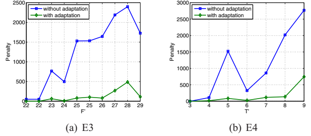
Figure 7. Two process types, without delays.
