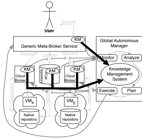
Figure 3. Hybrid integration of the knowledge management system
