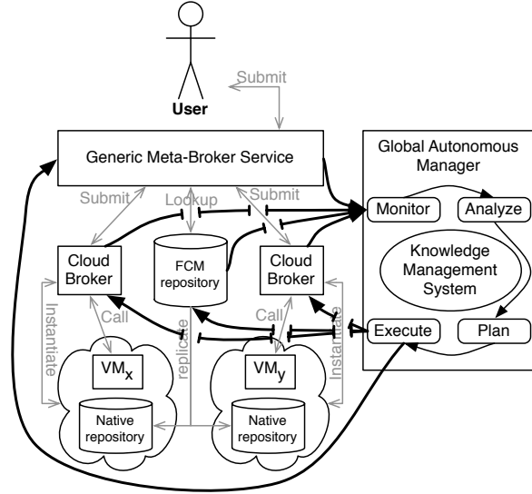
Figure 2. Global integration of the knowledge management system
