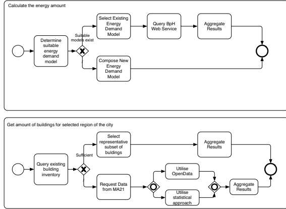
Fig. 2: Example of an analytical process in URBEM
