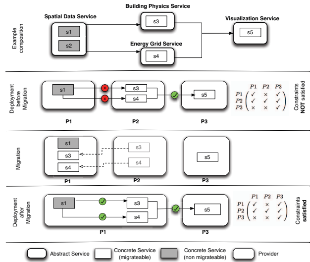
Fig. 3: Composition Scenario with Exchange Constraints and Service Migration
