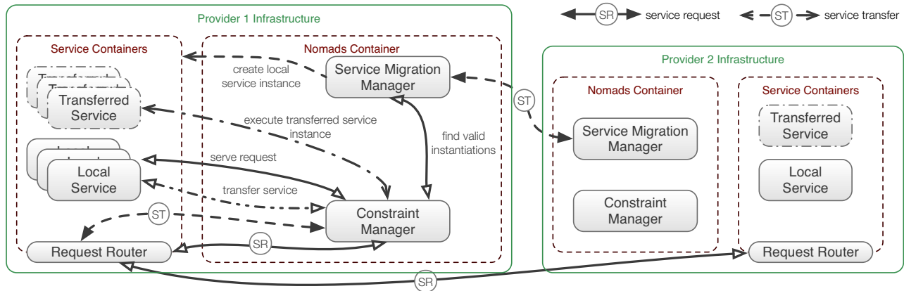
Fig. 5: Nomads Architecture
