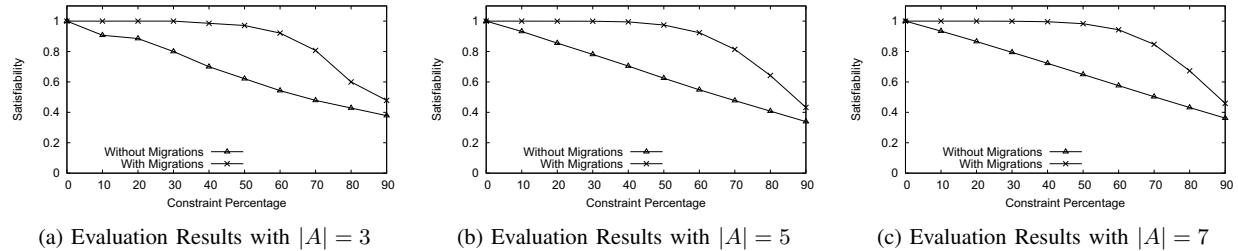
Fig. 8: Evaluation Results
