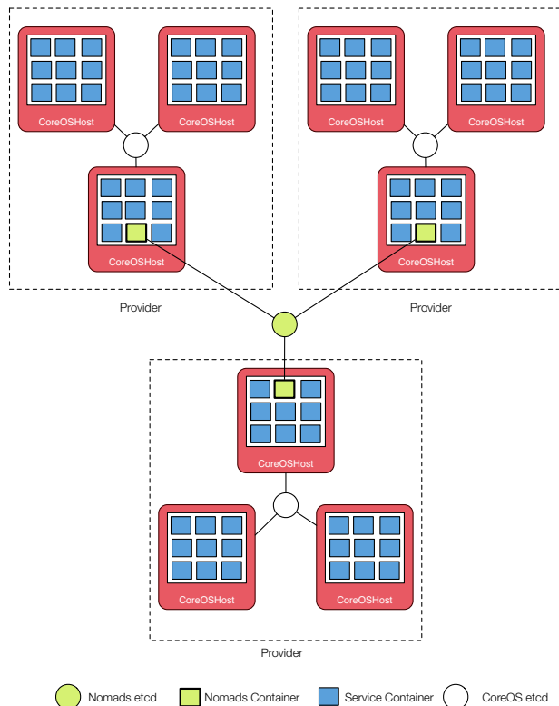
Fig. 7: Deployment for validation purposes
