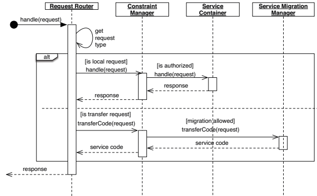
Fig. 6: Nomads Request Sequence Diagram
