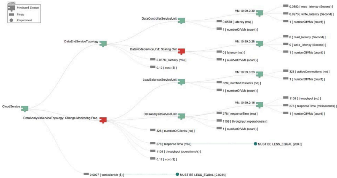
Fig. 6. Elasticity space monitoring integrated with control, deployment and testing events/metrics
