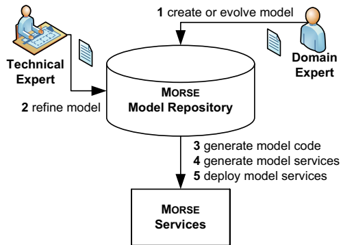
Figure 1. Generating MORSE Services for Models
