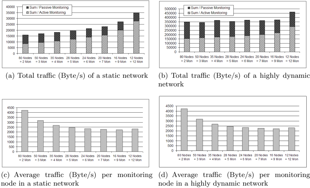
Fig. 5 Traffic of networks with various sizes of monitor groups
