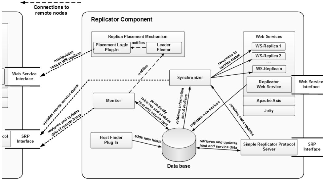
Fig. 1 Modular architecture of the replicator system
