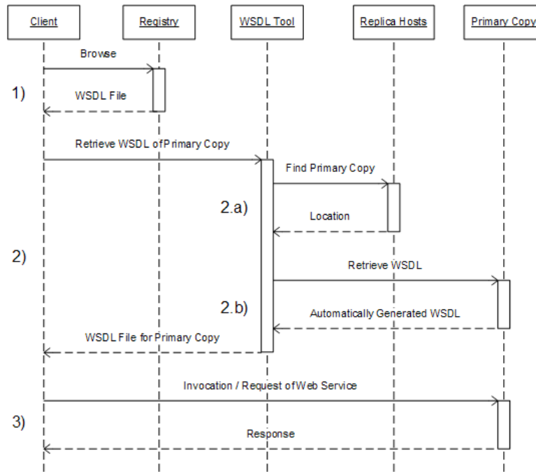
Fig. 4 Invocation of replicated Web services by using the WSDL-finder
