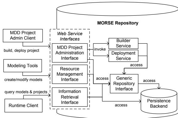
Figure 2. Architecture of the MORSE Repository
