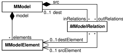
Figure 5. Model Element and Model Relations
