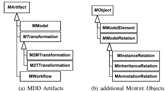
Figure 4. MDD Artifacts and additional MORSE Objects
