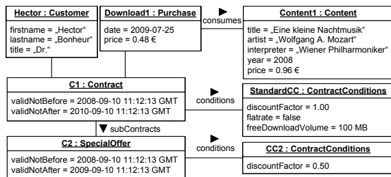
Figure 7. Payment Model Instances
