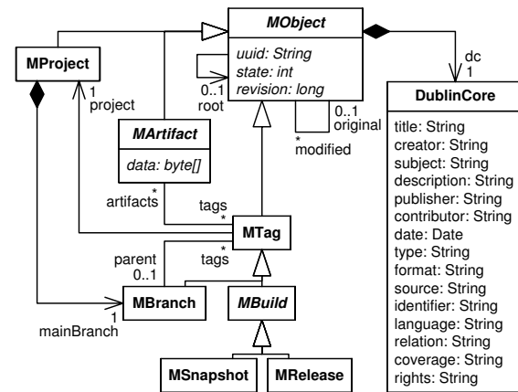
Figure 3. MORSE Objects and Projects
