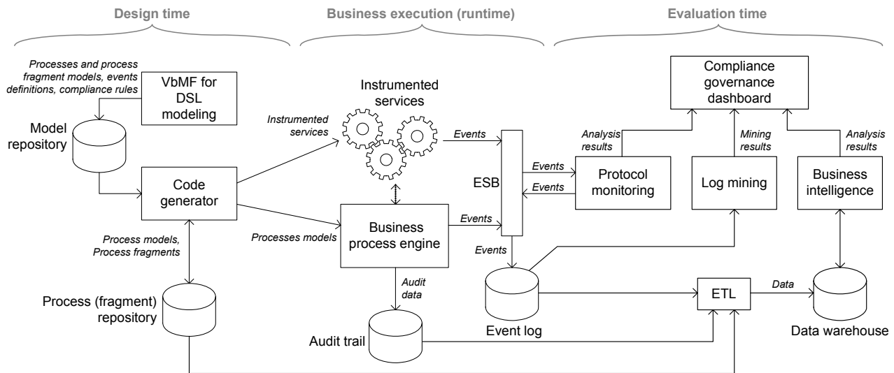
Figure 3 Overview of the COMPAS architecture for compliance governance in service-oriented architectures.
