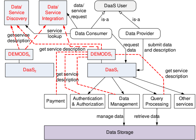
Fig. 1. DaaSes, users, and the use of DEMOS in a data marketplace
