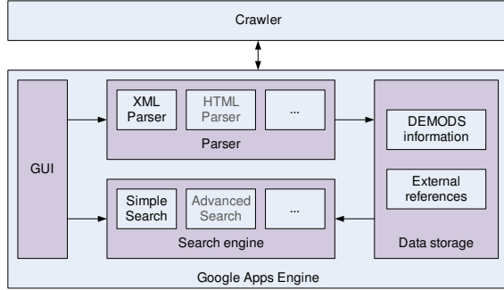
Fig. 3. A prototype of DEMODS Information Service
