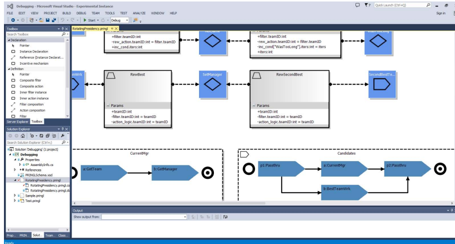
Fig. 5. Screenshot. Implementing a realistic incentive scheme using PRINGL Visual Studio environment.
