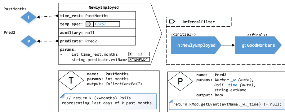
Fig. 3. A CompositeWorkerFilter for referral bonuses
