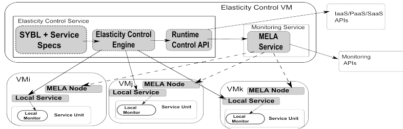
Fig. 1: Monitoring and controlling elastic cloud services
