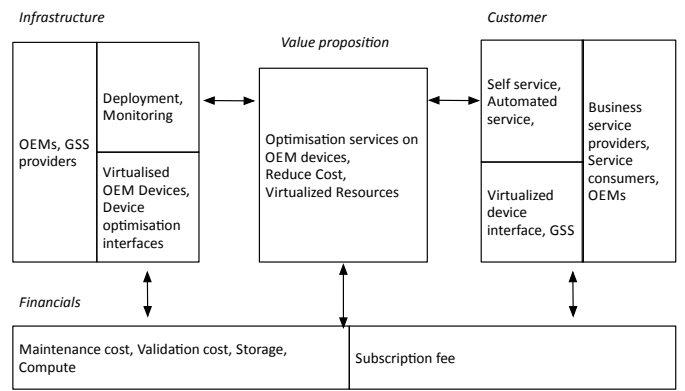
Fig. 3. Infrastructure services
