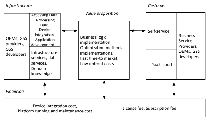
Fig. 4. Platform services
